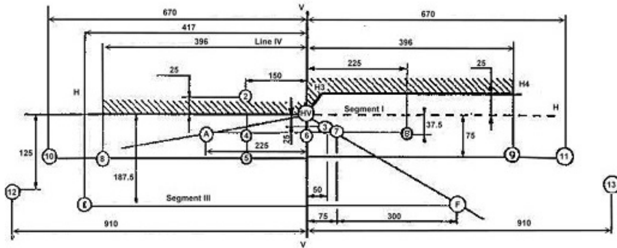
Figure 2.Measuring screen 2
