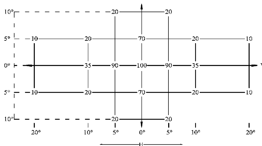
Figure 1. Light distribution
