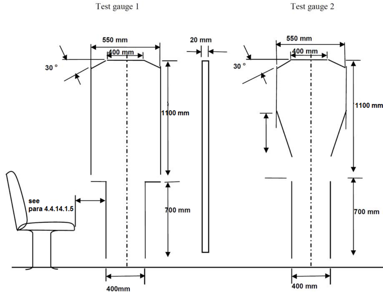
Figure 1 Test gauge
