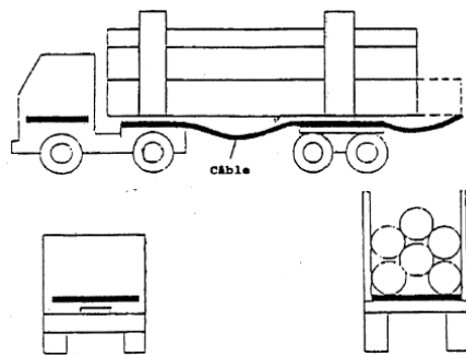
3-2.6.14.4.2 Examples of retro-reflective contour markings (with distinctive markings and graphics)
