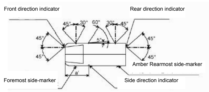
Fig 4. Horizontal angle of front/rear direction-indicator lamp and side-marker lamp
