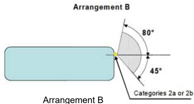
Fig 3. The visibility of direction-indicator lamp -- Horizontal angle
