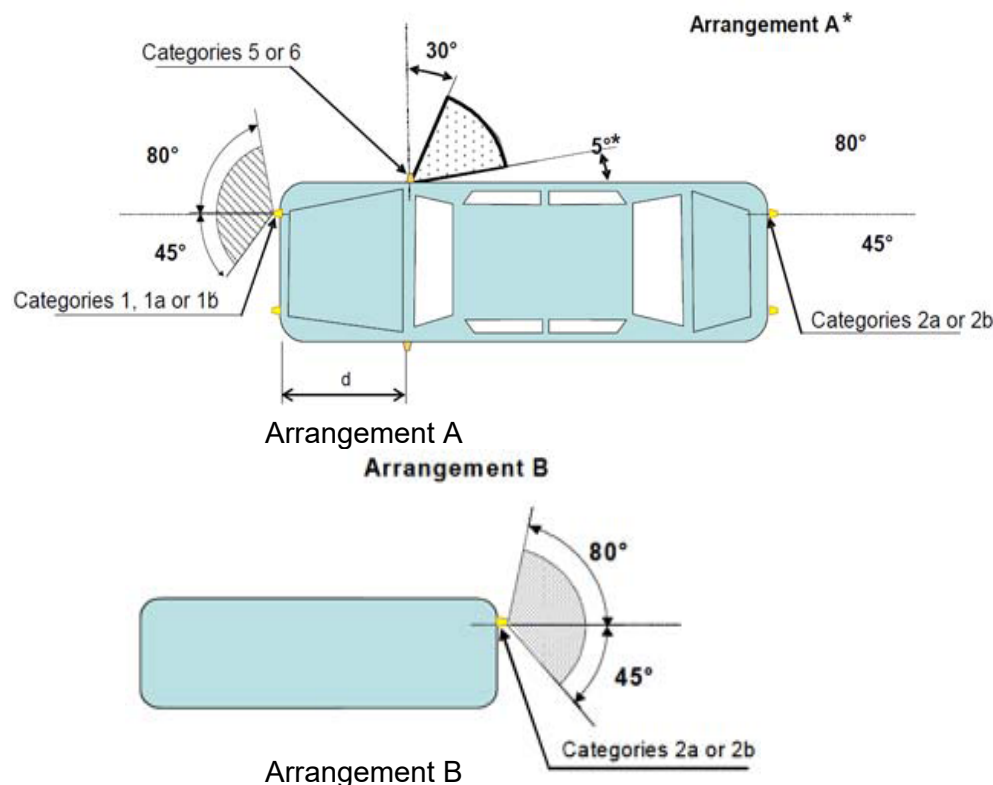
Fig 3. The visibility of direction-indicator lamp -- Horizontal angle
