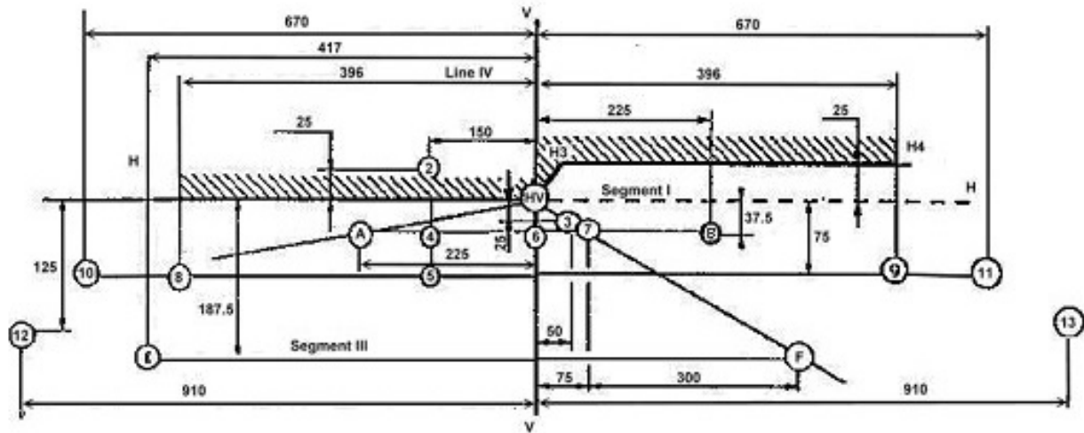
Figure 2.Measuring screen 2
