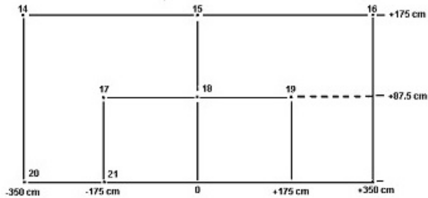
Figure 3. Measuring points for illumination values
