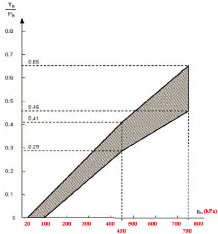
Diagram 4A Semi-Trailers
