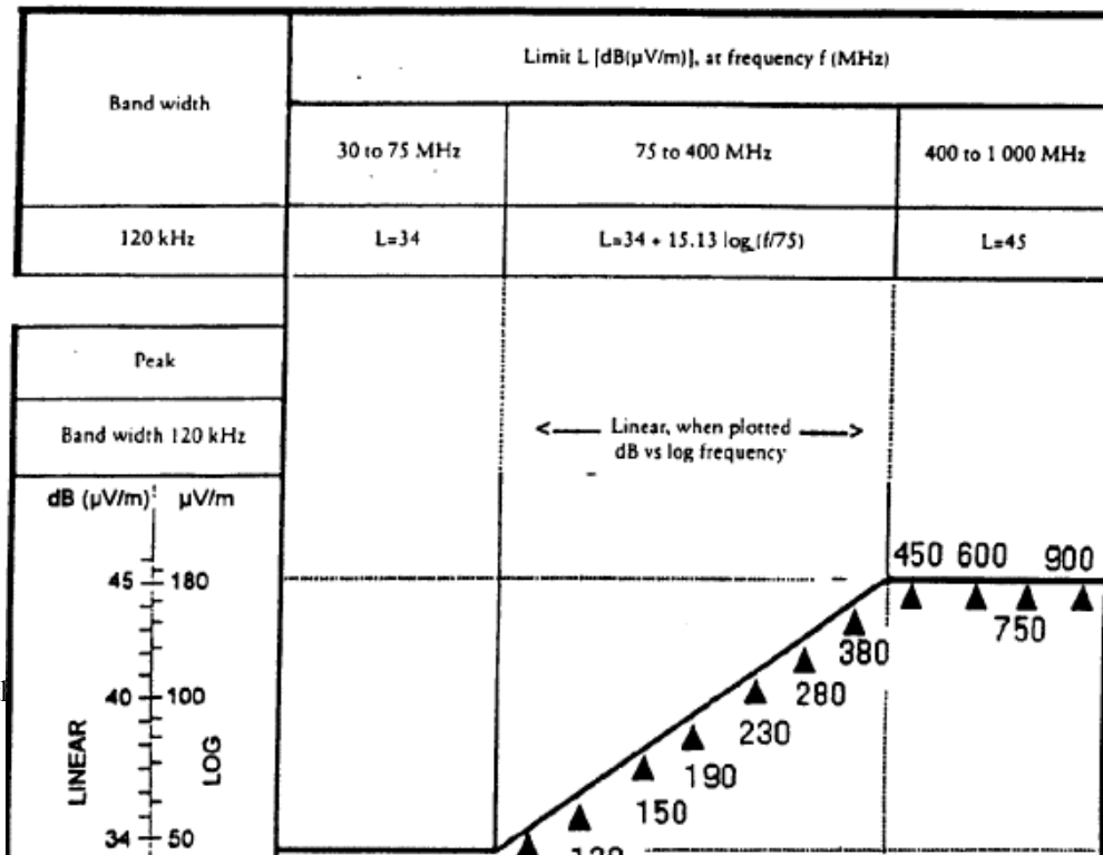
Vehicle narrowband reference limits Antenna-vehicle separation: 3m
