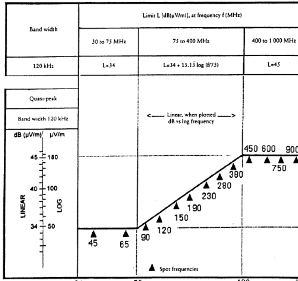
Vehicle broadband reference limits Antenna-vehicle separation: 10 m
