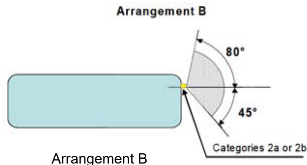
Fig 3. The visibility of direction-indicator lamp -- Horizontal angle
