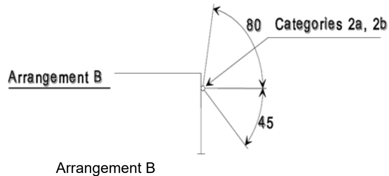
Fig 3. The visibility of direction-indicator lamp -- Horizontal angle
