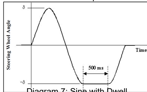
Diagram 7: Sine with Dwell
