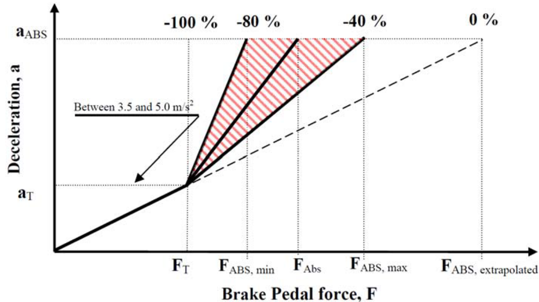
Figure 8a: Pedal force characteristic needed in order to achieve maximum deceleration with category “A” BAS
