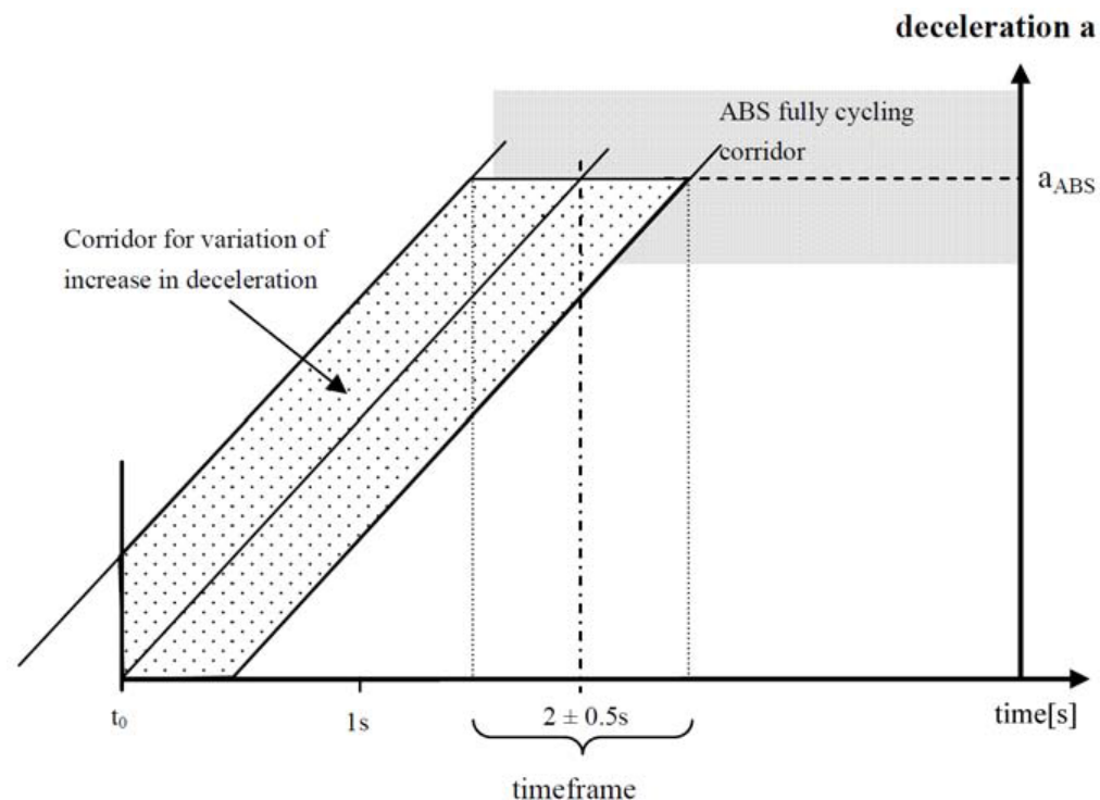
Figure 10: Deceleration corridor for determination of F_{ABS} and a_{ABS}
