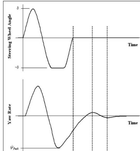
Diagram 6: Steering wheel position and yaw velocity information used to assess lateral stability
