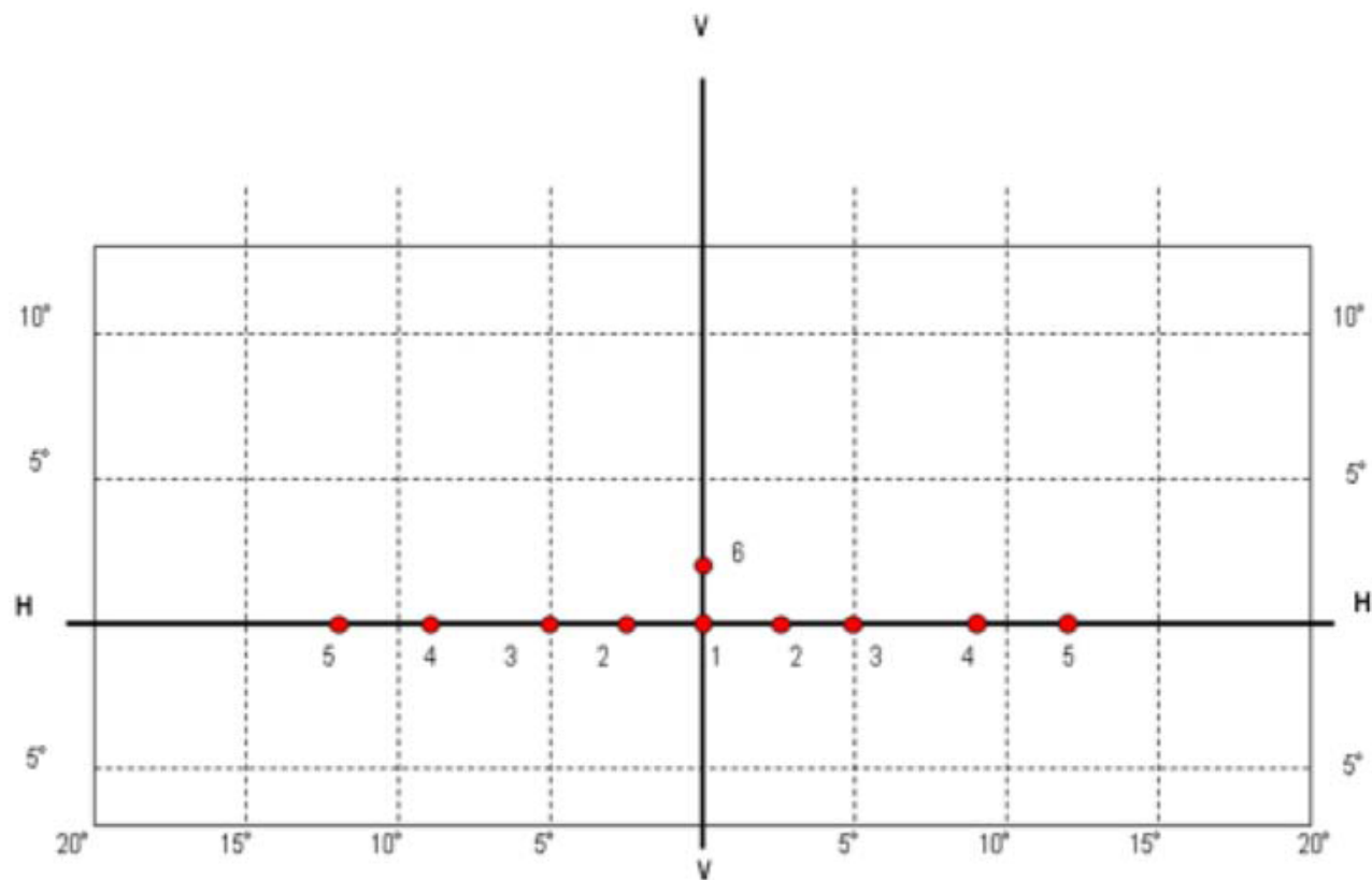
Figure 6: Primary driving beam - position of test points
