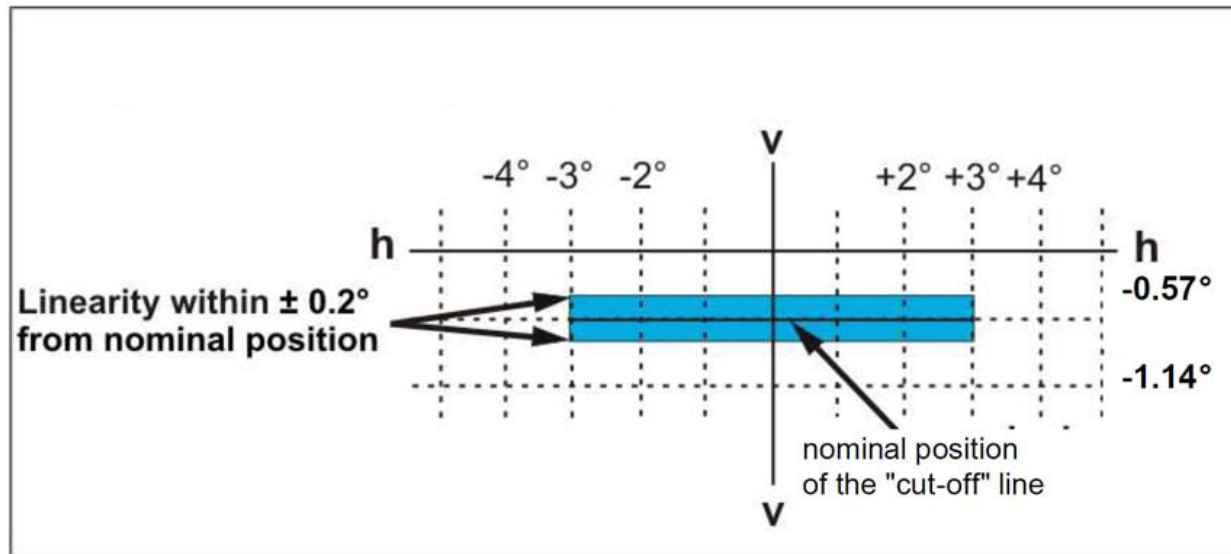
Figure 5: Shape and position of the "cut-off" line
