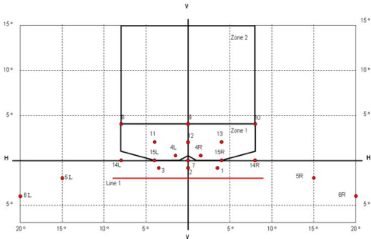
Figure 4-3: Passing beam - position of test points and zones for Classes C, D and E headlamp(s):
