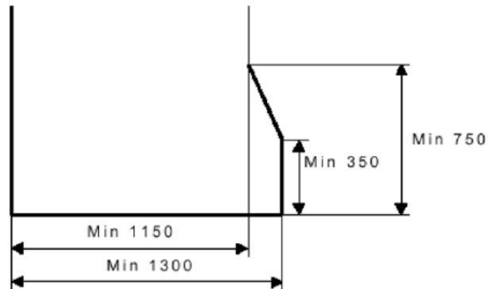
Figure 4: Minimum clear space for the wheelchair user at the wheelchair space
