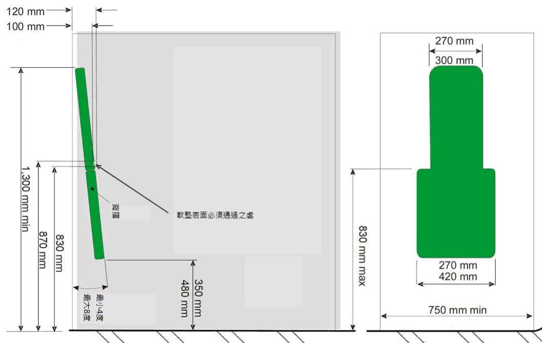
Figure 7 Example of a backrest for a rearward-facing wheelchair
