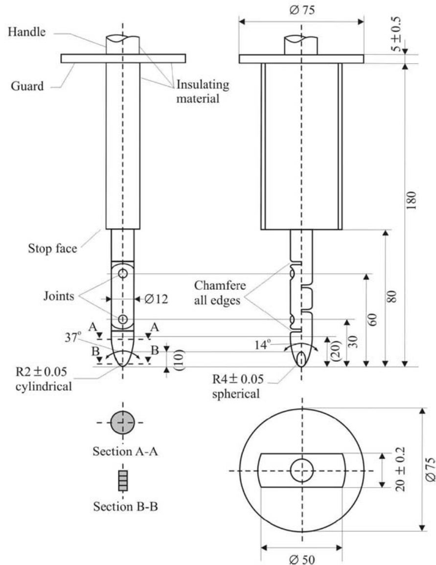
Figure 5: Jointed test finger (degree IPXXB)
