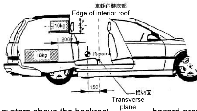
Fig. 3 Testing of a partitioning system above the backrest regarding hazard-prevention from the moving luggage
