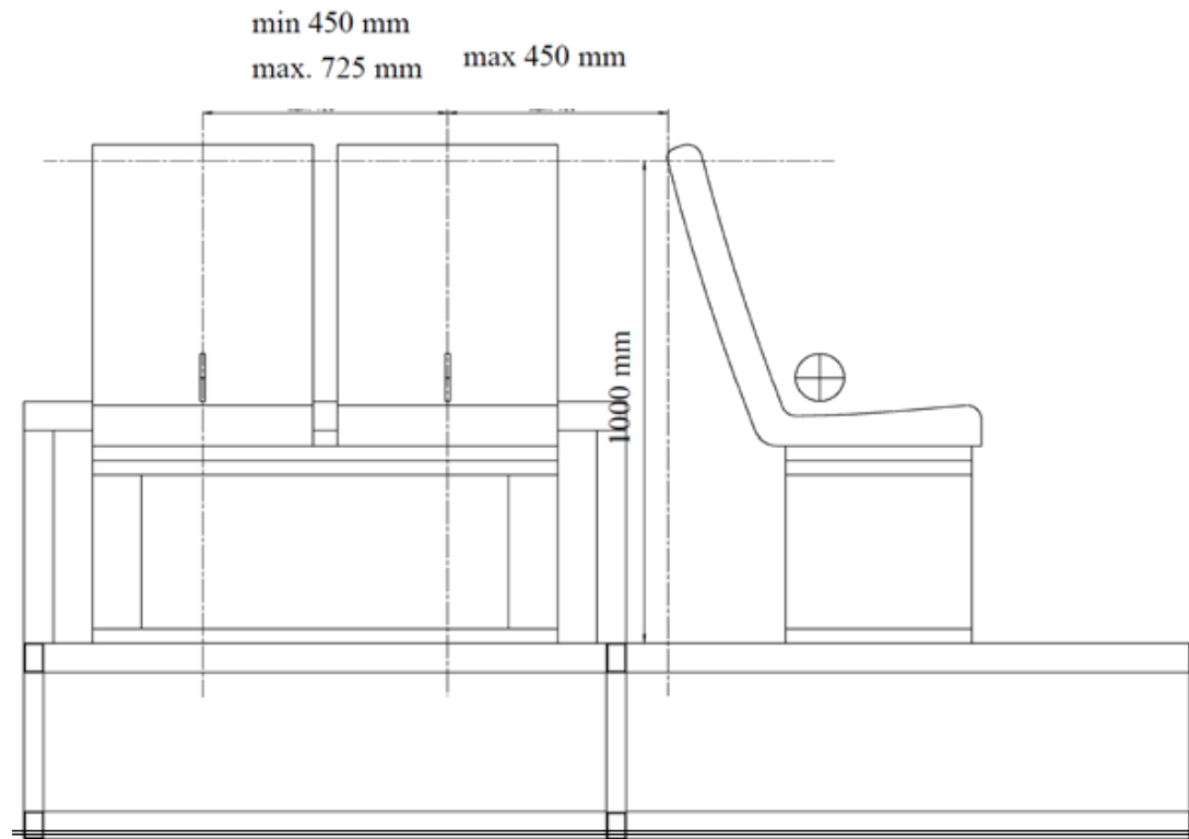
Figure 7: Positioning requirements for side-facing seats
