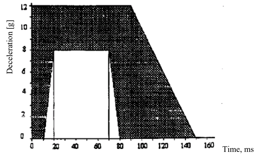
Fig. 5 Trolley's impacting acceleration/deceleration.
