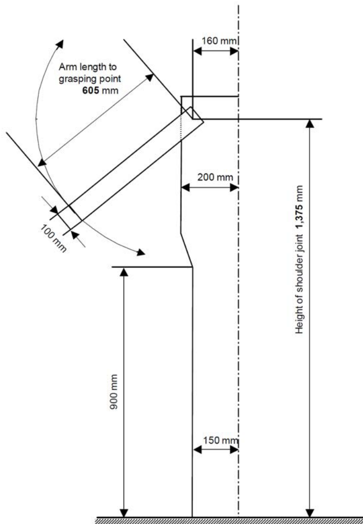
Figure 9: Testing device for siting of handholds
