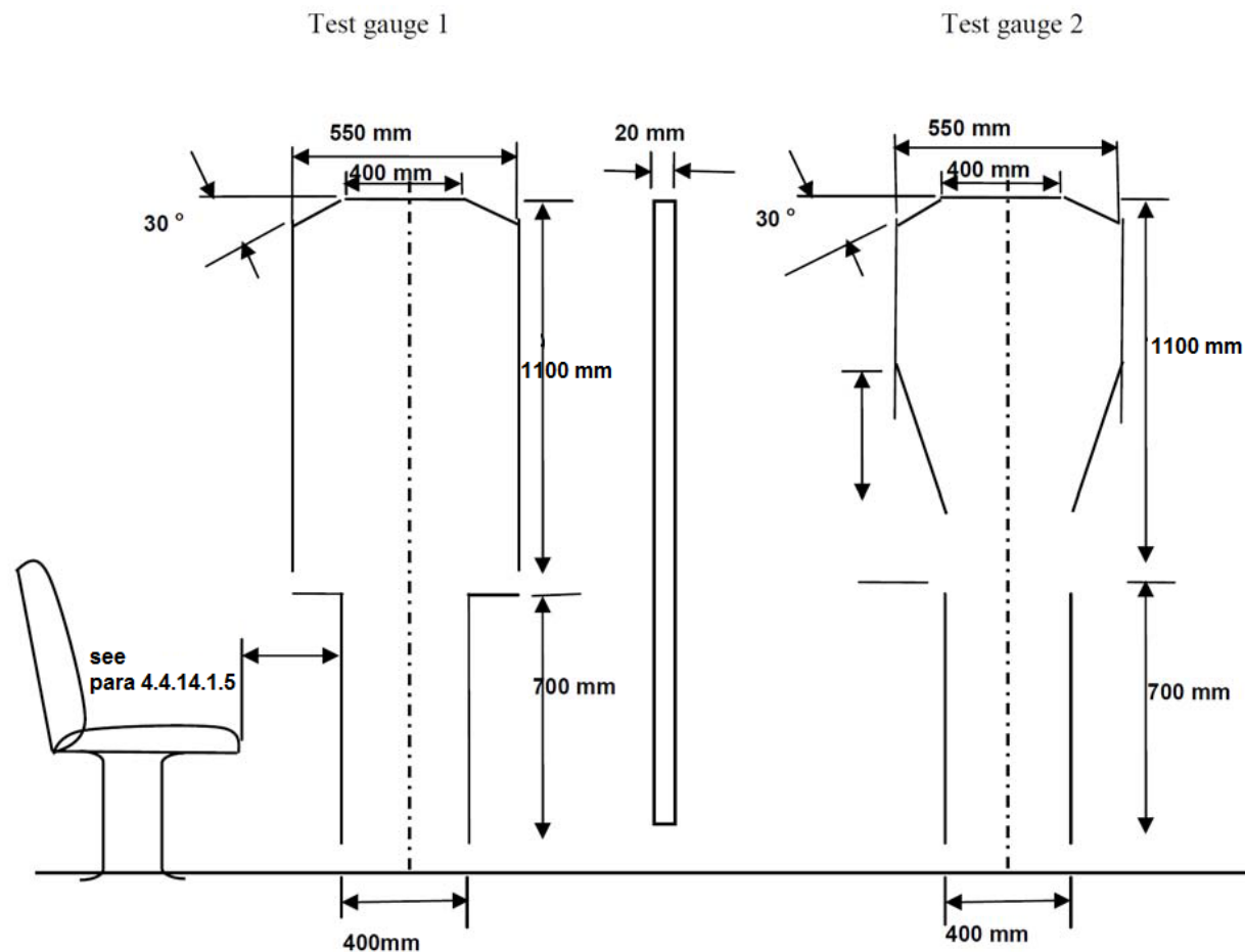
Figure 4 Test gauge
