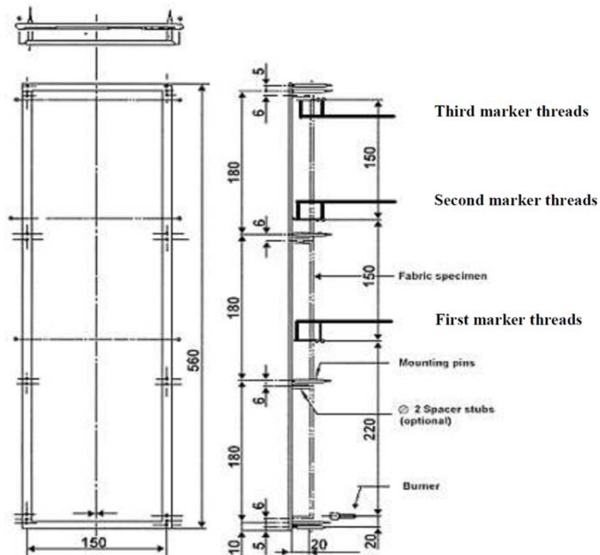
Figure 4: Burner ignition location
