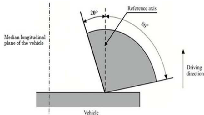
Figure 2-2 Horizontal angles for Front position lamp fitted to L vehicles with a pair of lamps of paragraph 34.4.4.2.
