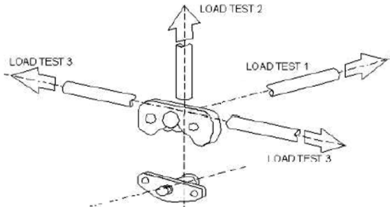
Figure 4 - Door Static Load Test Directions
