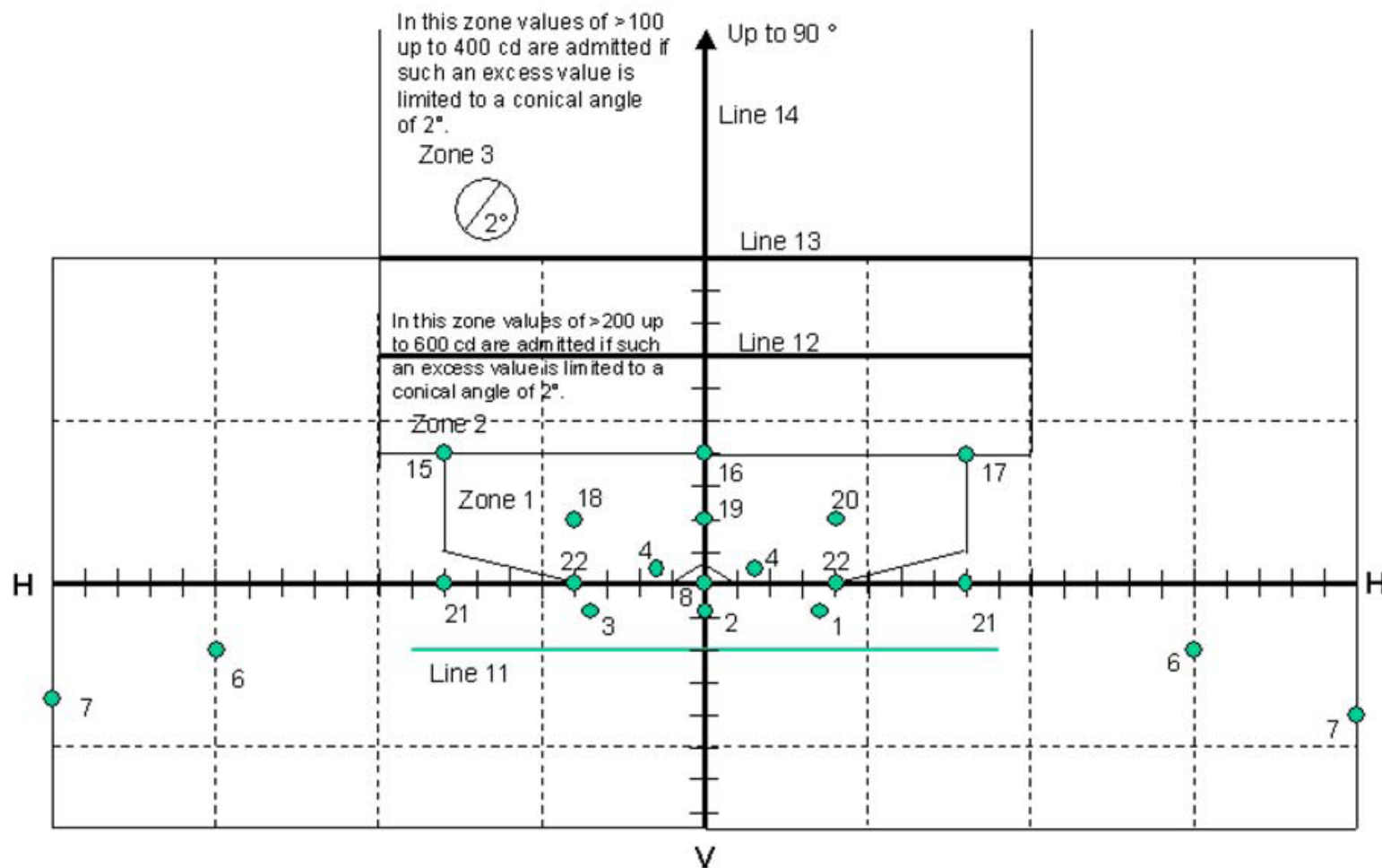
Figure 7 : (Dimensions in mm with screen at 25 m distance) Note: The luminous intensity of zones 2 and 3 above are not applied to Class E.
