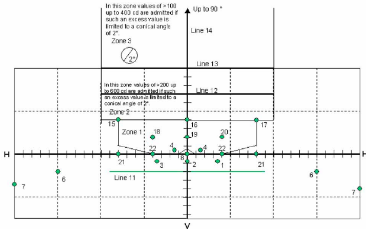
Figure 2. Measuring screen for symmetrical headlamp
