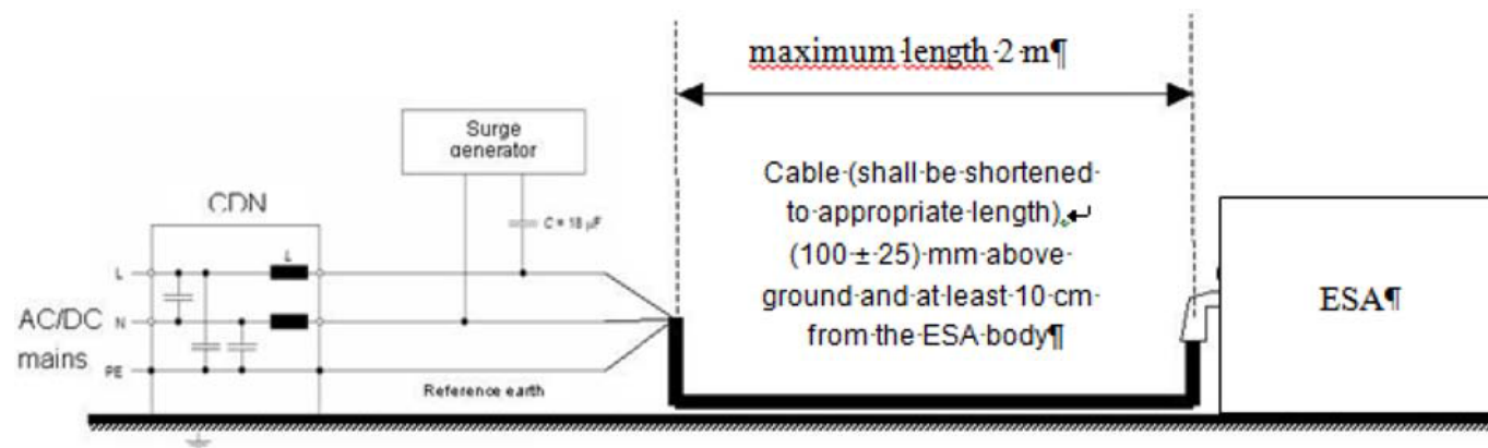
Figure 39: ESA in configuration "REESS charging mode coupled to the power grid" - Coupling between lines for DC or AC (single phase) power lines
