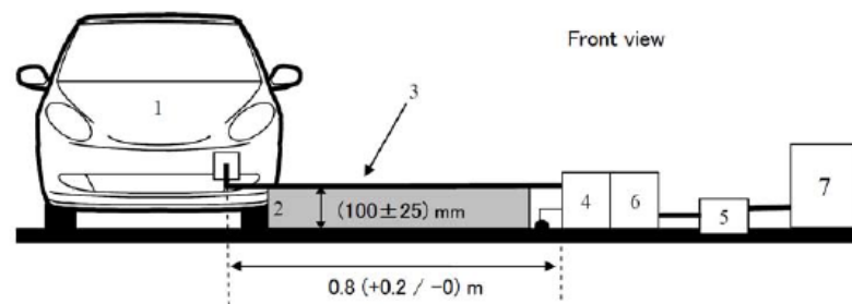
Figure 15-3: Vehicle in configuration "REESS charging mode coupled to the power grid"
