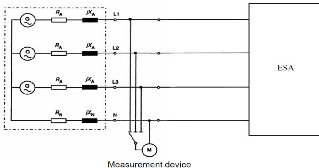
Figure 35-2: ESA in configuration "REESS charging mode coupled to the power grid" - Three-phase test set-up
