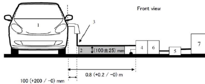
Figure 15-2: Vehicle in configuration "REESS charging mode coupled to the power grid"
