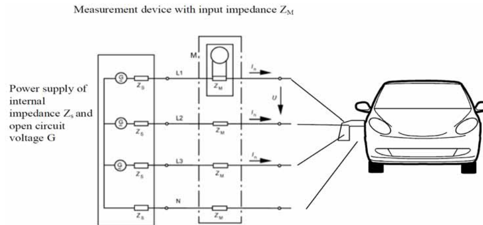
Figure 23: Vehicle in configuration "REESS charging mode coupled to the power grid" - Three-phase charger test set-up
