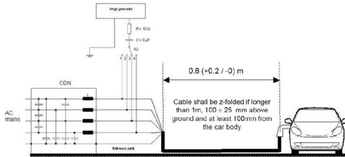
Figure 32: Vehicle in configuration "REESS charging mode coupled to the power grid" – Coupling between each line and earth for AC (three phases) power lines
