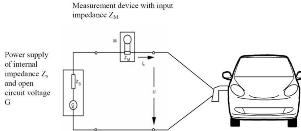
Figure 22: Vehicle in configuration "REESS charging mode coupled to the power grid" - Single phase charger test set-up
