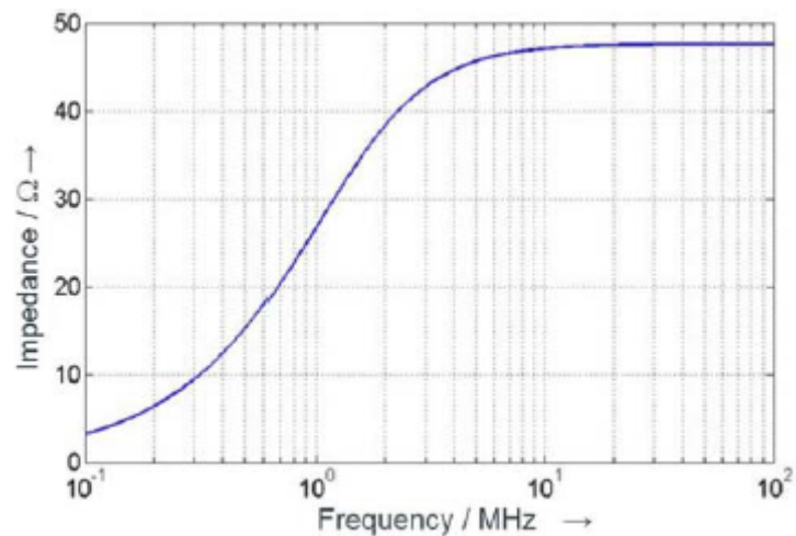
Figure 8: Impedance of HV artificial network
