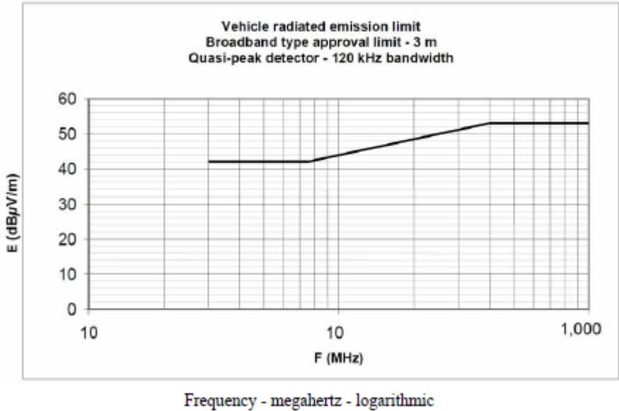
( See paragraph 4.2.2.2 of this Regulation ) Figure 2: Vehicle broadband reference limits ( Antenna-vehicle separation :3 m )
