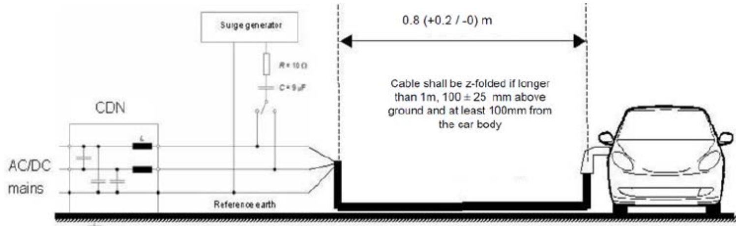
Figure 30: Vehicle in configuration "REESS charging mode coupled to the power grid" – Coupling between each line and earth for DC or AC (single phase) power lines
