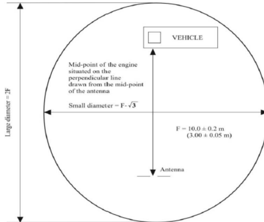
Figure11: Clear horizontal surface free of electromagnetic reflection delimitation of the surface defined by an ellipse
