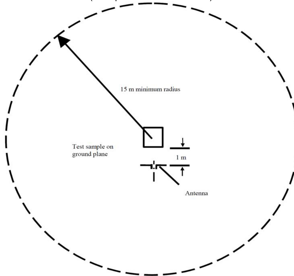
Figure13: Test configuration for ESAs involved in "REESS charging mode coupled to the power grid" (Example for biconical antenna)
