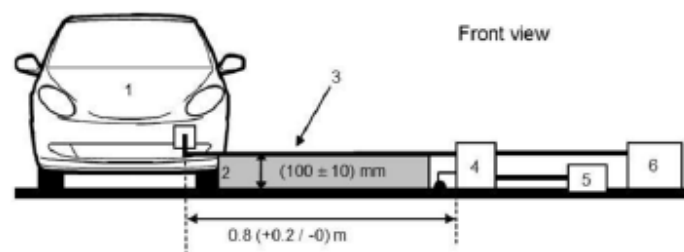
Figure 25-1: Vehicle in configuration "REESS charging mode coupled to the power grid"
